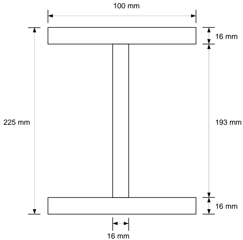
Figure 3.15 – 350W Section
