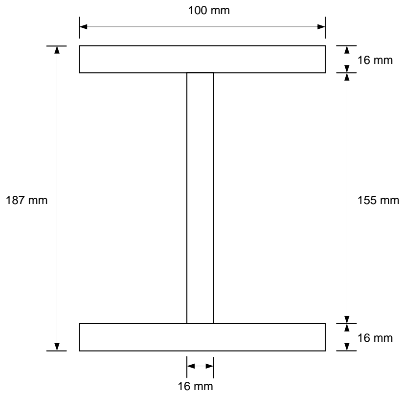
Figure 3.16 – 460W Section
