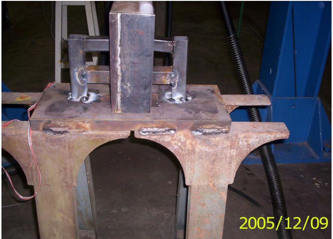
Figure 3.13 – Bracing of the specimen
