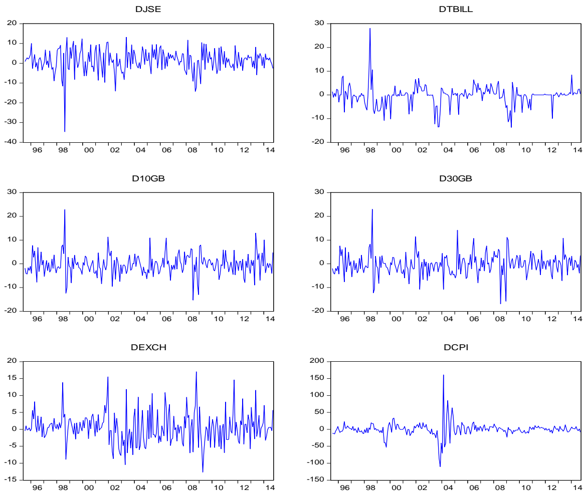
Figure 3: Time plot of the variables in first difference
