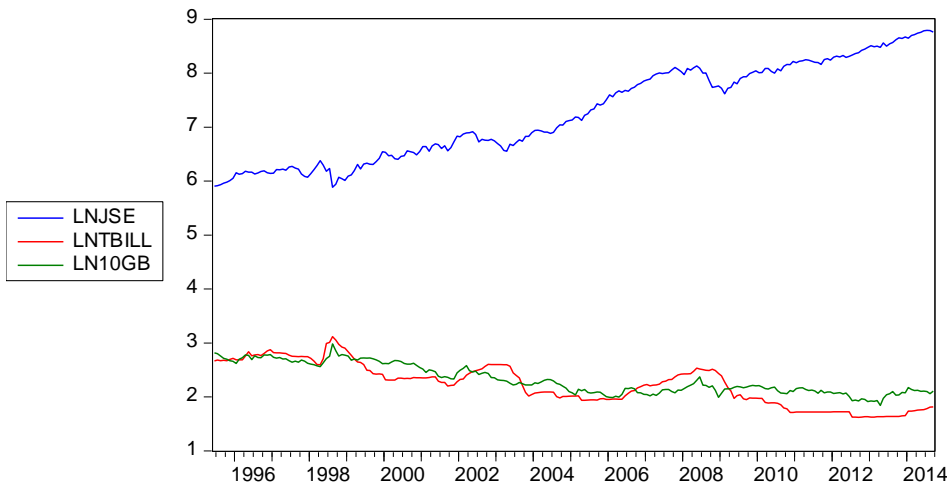
Figure 1: Trend analysis
