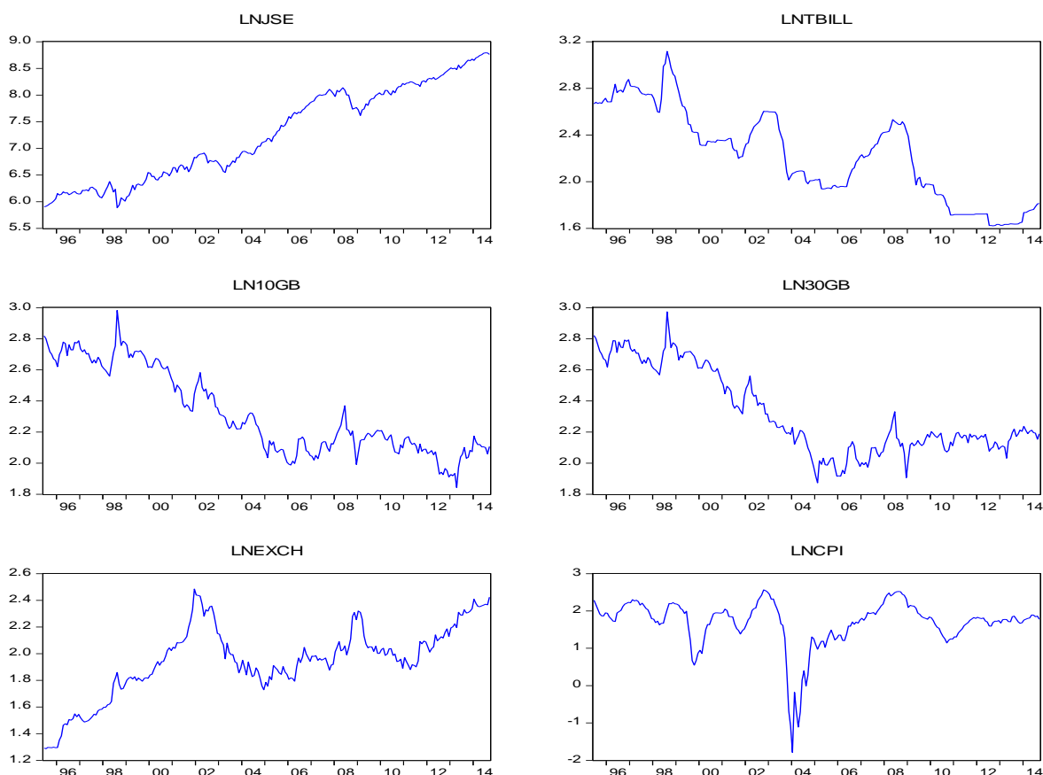
Fig 2: Time series Plots of the logarithms of the variables.
