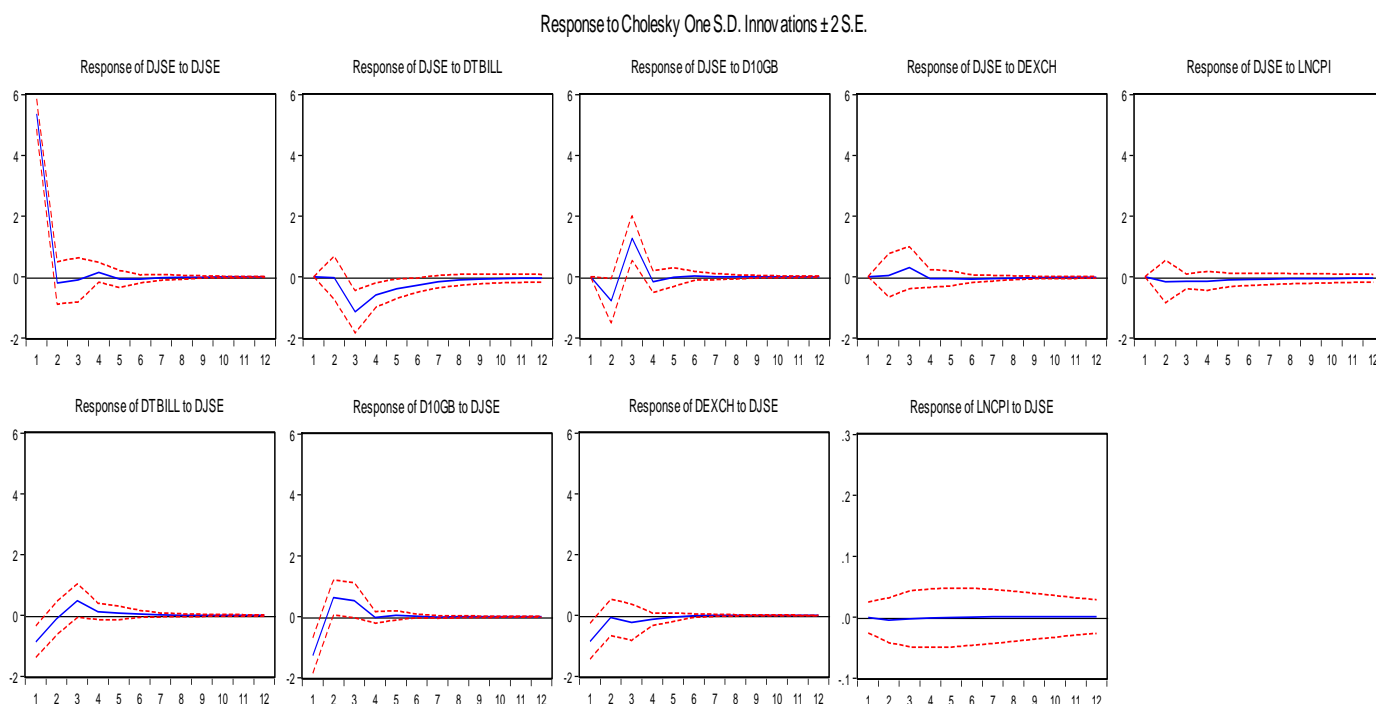
Figure 4: Impulse Response Functions
