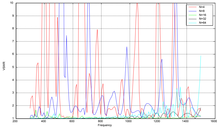
Figure 2.3 Variation of VSWR with frequency for fixed values of N
