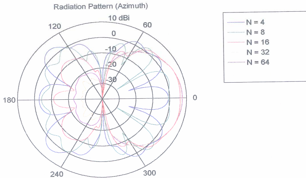
Fig 2.5: Variation of radiation pattern with values of number of element 'N'.
