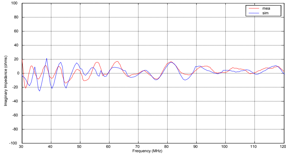
Figure 2.2 Plot of imaginary input resistance variation with frequency N = 15 , L = 1.5\text{m} , \tau = 0.89 and \sigma = 0.073
