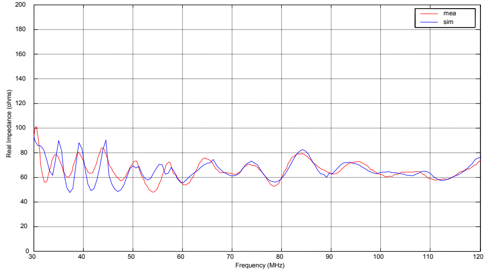
Figure 2.1 Plot of real input impedance variation with Frequency, L=1.5\text{m} , N=15 , \tau = 0.89 and \sigma = 0.073
