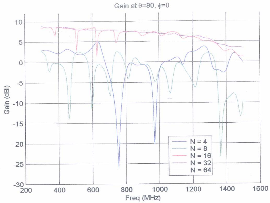
Fig 2.4: Variation of gain with frequency for values of number of element 'N'.
