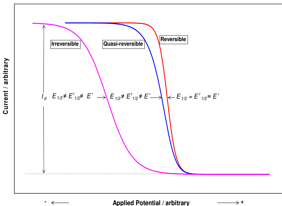
Figure 3.3: Schematic comparison of DC polarograms corresponding to reversible, quasi-reversible, and irreversible reduction processes. E_{1/2} and E_{1/2}^r stand for observed half-wave potential and reversible half-wave potential, respectively. E^\circ stands for the standard reduction potential.
