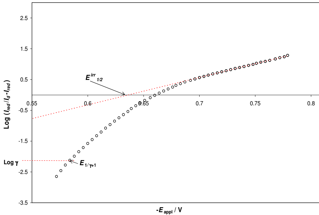
Figure 3.9: Logarithmic analysis of a quasi-reversible DC polarographic wave using the Matsuda–Ayabe method (see text for details).
