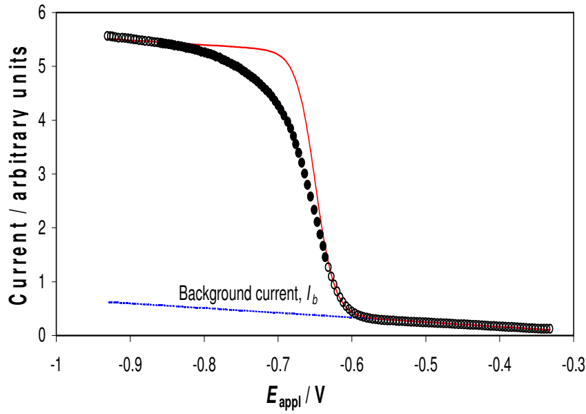
Figure 3.8: An example of the analysis of a quasi-reversible DC polarogram for the reduction of \text{Cd}^{2+} at 25 °C in 0.5 M \text{NaNO}_3 , in the presence of the ligand sarcosine, using the Cukrowski's curve-fitting method. Open circles (o) represent recorded experimental points; the solid line represents the computed DC polarogram obtained from the curve-fitting operation (see text for details).
