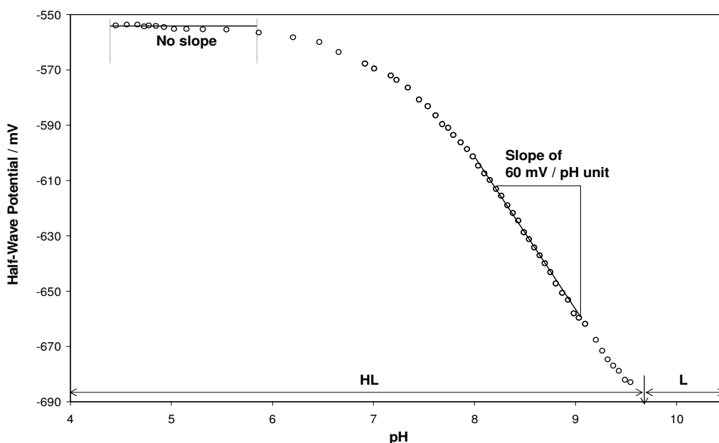
Figure 3.1: A typical relationship of variation in half-wave potential for \text{Cd}^{2+} , in the presence of the protic ligand glycine, as a function of pH.
