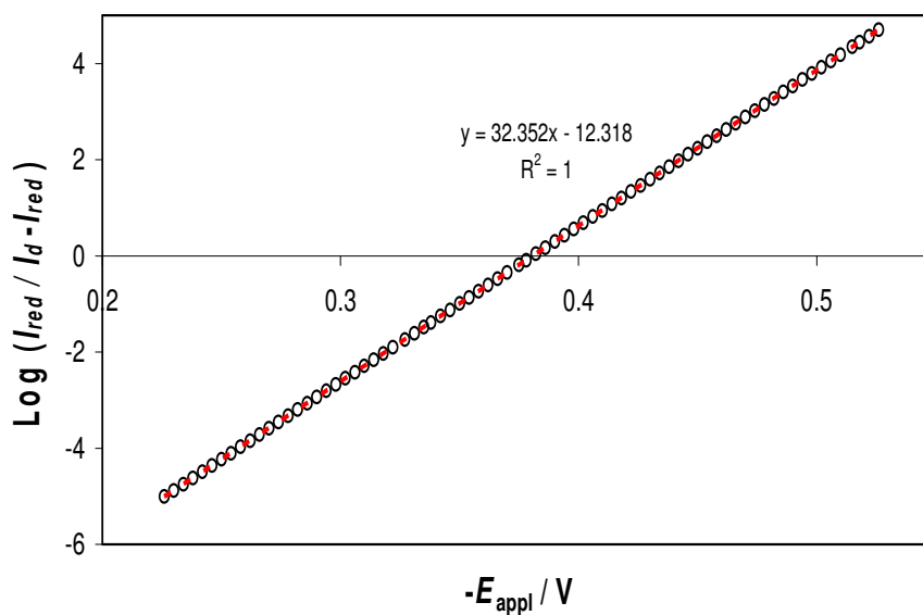
Figure 3.5: A logarithmic analysis corresponding to the DC polarogram for the reversible reduction of \text{Pb}^{2+} at 25 °C in 0.5 M \text{NaNO}_3 shown in Figure 3.4. Circles indicate the experimental points while the dashed line is a fitted linear trendline. See text for interpretation details.
