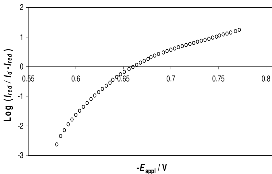
Figure 3.7: A logarithmic analysis of the DC polarogram seen in Figure 3.6. The curved logarithmic plot indicates a quasi-reversible reduction process.
