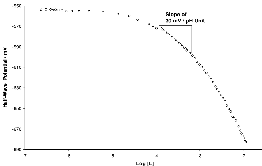
Figure 3.2: An example of a typical relationship of variation in half-wave potential as a function of \text{Log } [L] .
