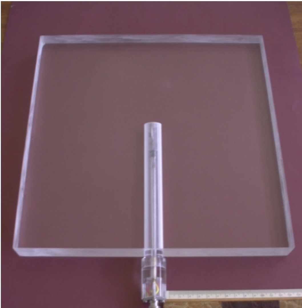
Figure 5.23: Photograph of Mark IIA in its customized Perspex phantom.
