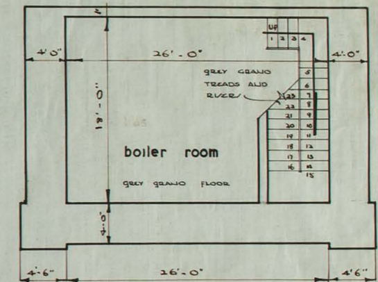
basement plan
