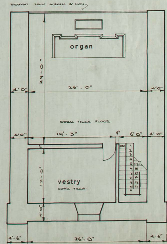
plan of transept
