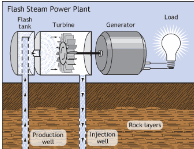
Figure 20: Flash Steam Power Plant Diagram [78]
