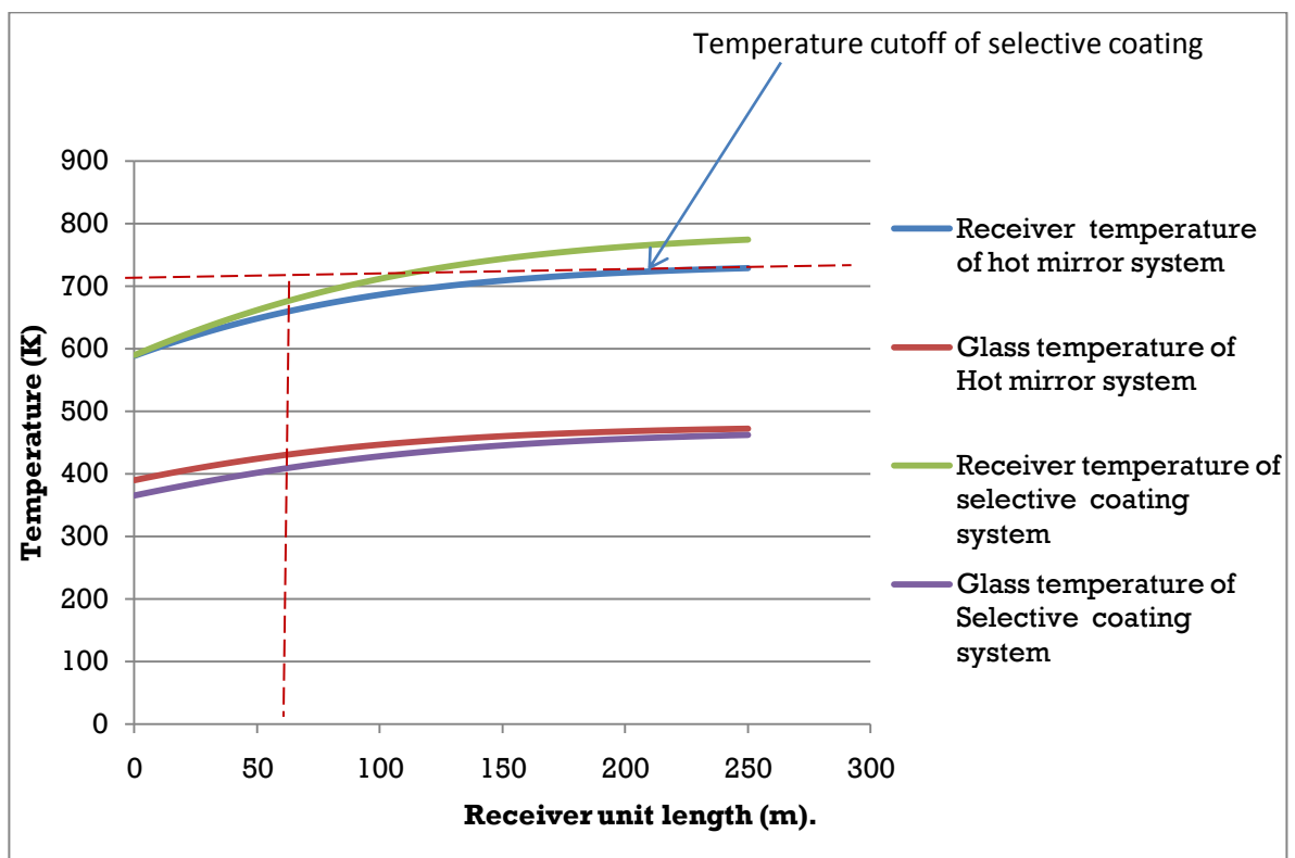
Graph 1: Comparison between selective coating and hot mirror temperature of glass cover and hot mirror. Although the graph for selective coating is shown along the entire length of the receiver unit, it is understood that this graph terminates at the dotted vertical line, due to thermal decomposition.
