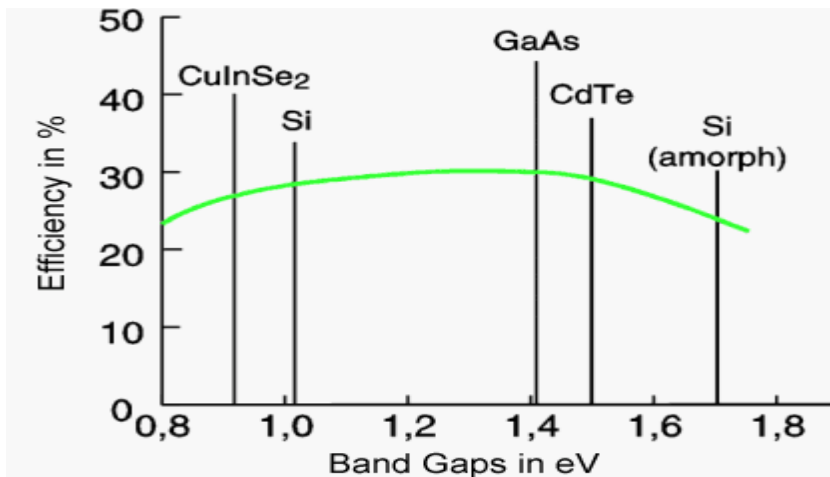
Figure 5: Theoretical maximum levels of efficiency of various solar cells at standards conditions [24].
