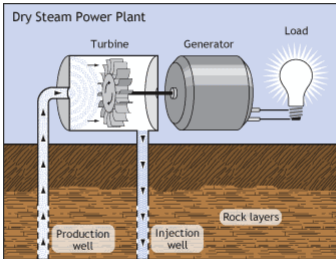
Figure 19 : Dry steam Power plant diagrams [78]
