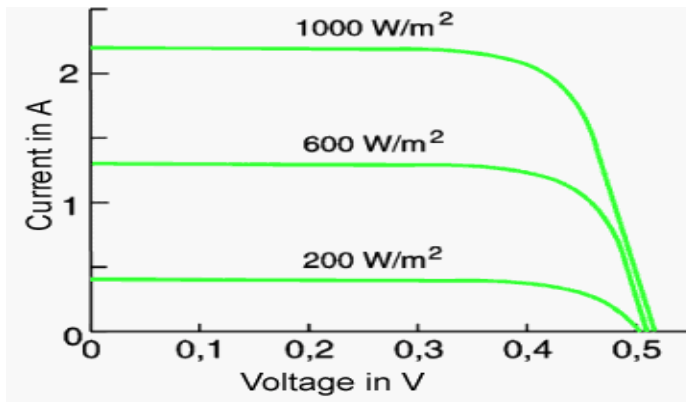
Figure 3: An example of current –voltage characteristic line of Si solar cell [14]
