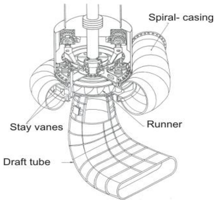
Figure 16: Francis turbine [55]
