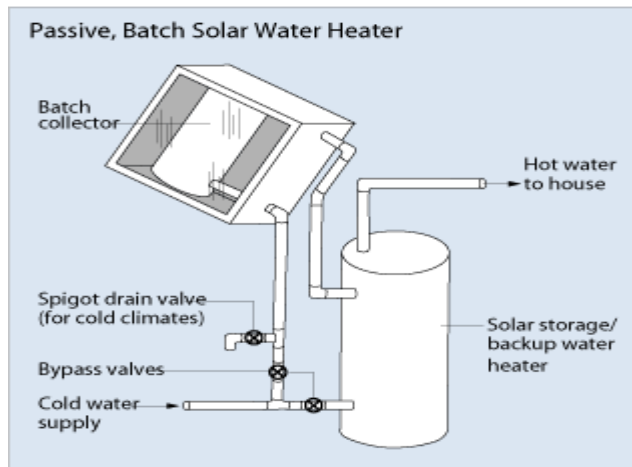
Figure 6: Passive, Batch solar water heater [23]
