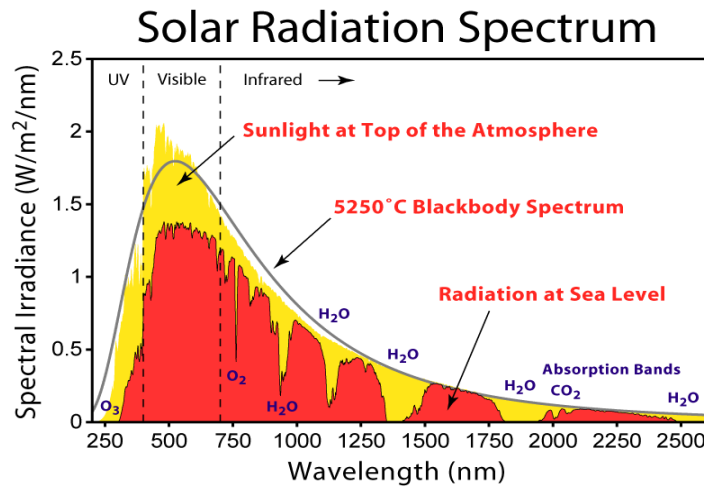
Figure 1 : Solar radiation spectrum [8]
