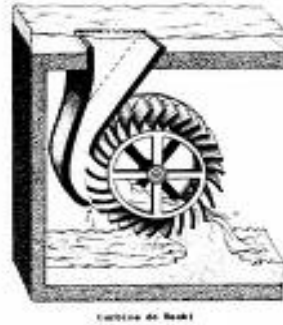
Figure 14: Cross flow turbine [54]
