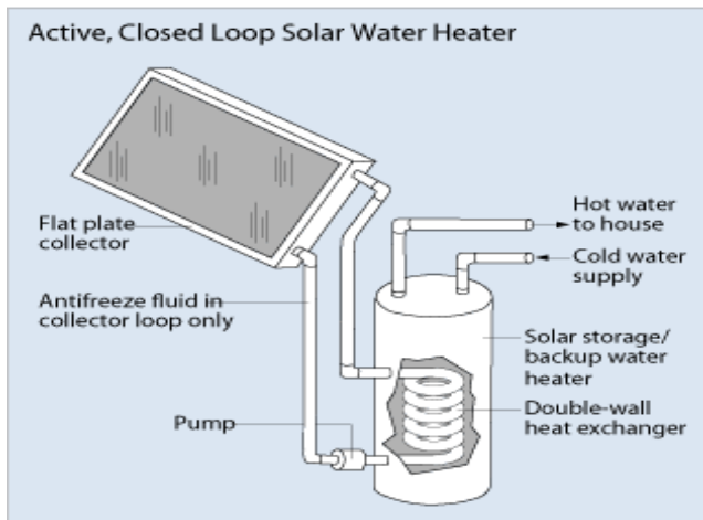
Figure7: Active, closed loop solar water heater [23]
