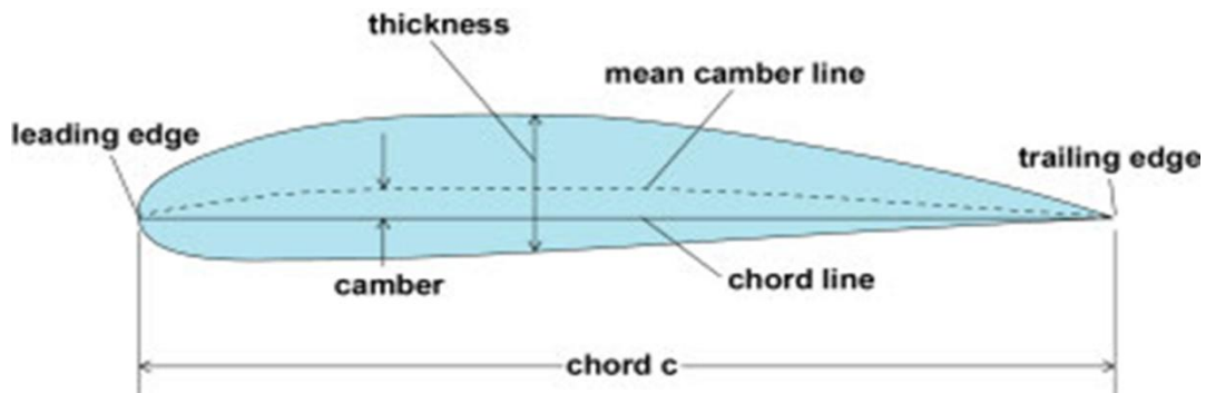
Figure 24: Airfoils [15]
