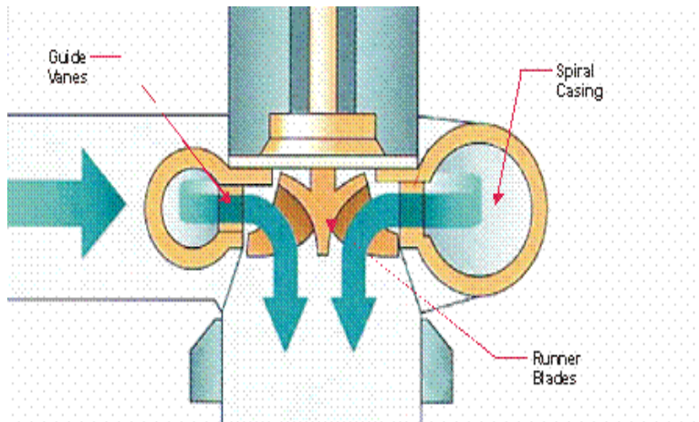
Figure 15: propeller turbine (Kaplan type) [51a]
