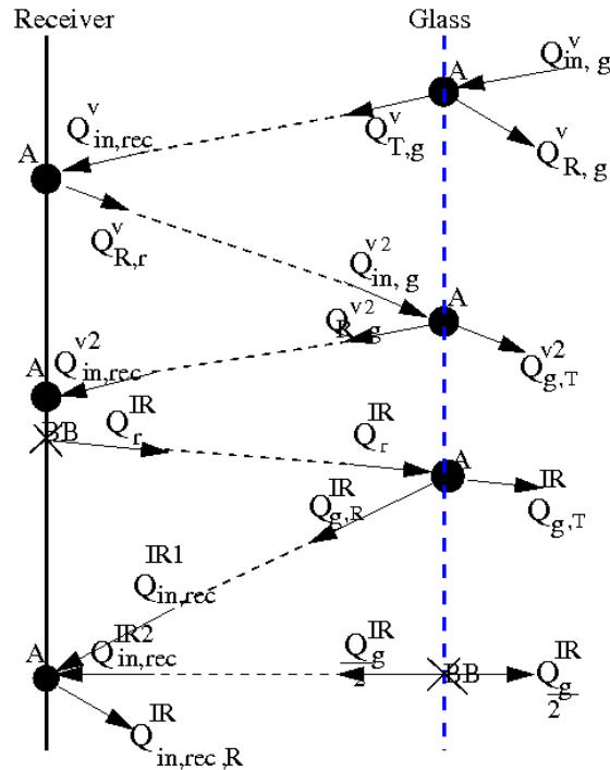
Figure 30: Radiation types falling on our system surfaces. At every node there is a chance for reflection, transmission and absorption. The shot-dashed lines connecting nodes refer mainly to the fact that output of one becomes input of the next, e.g. Q_{in,rec}^v = Q_{T,g}^v .
