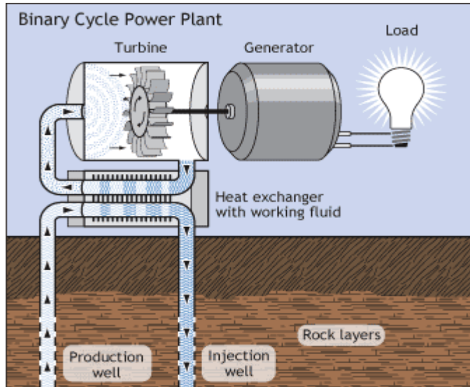
Figure 21 : Binary cycle Power Plant diagram [78]
