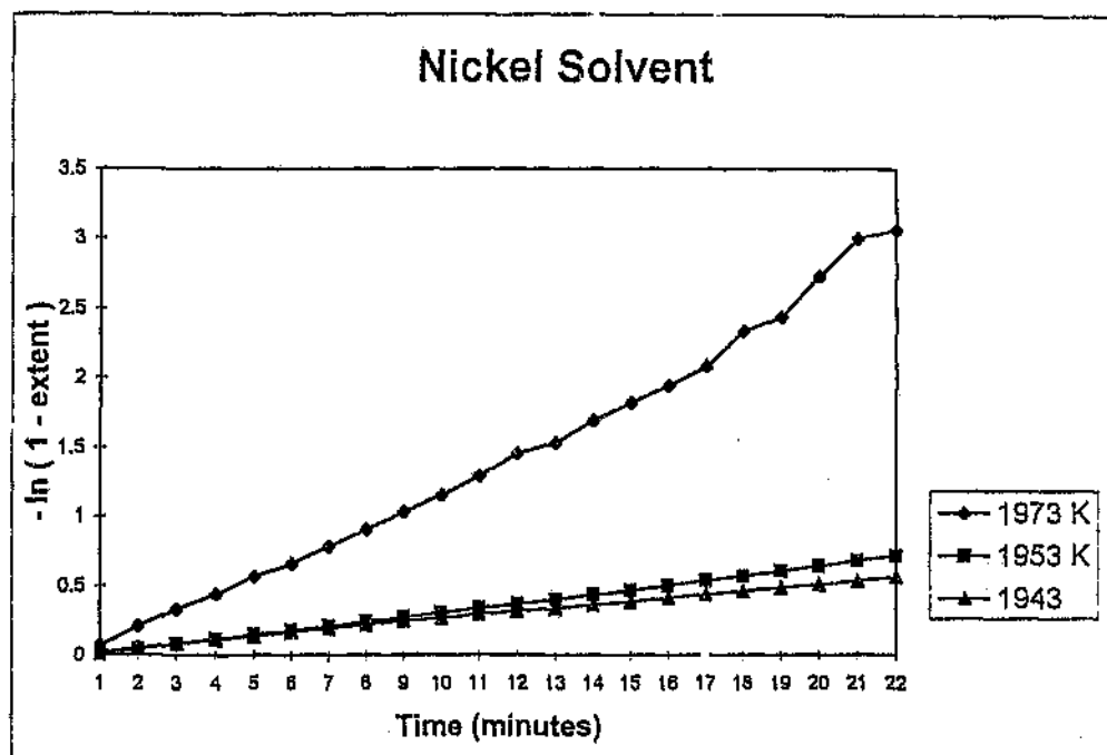
Figure 4.7 Extent of Reaction vs. Time in Nickel Solvent
