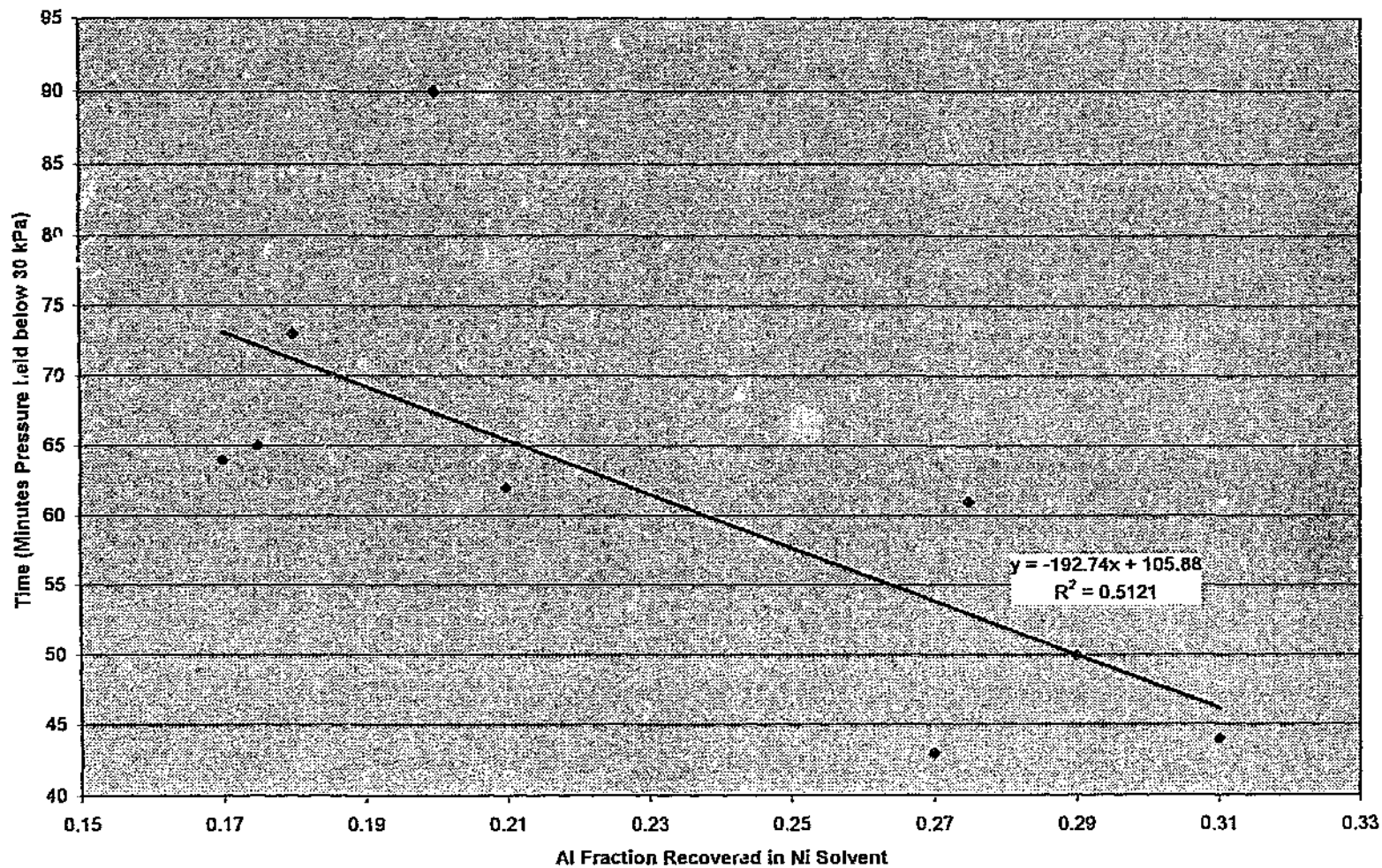
Figure 4.12 EFFECT OF PRESSURE ON VAPORISATION OF Al
