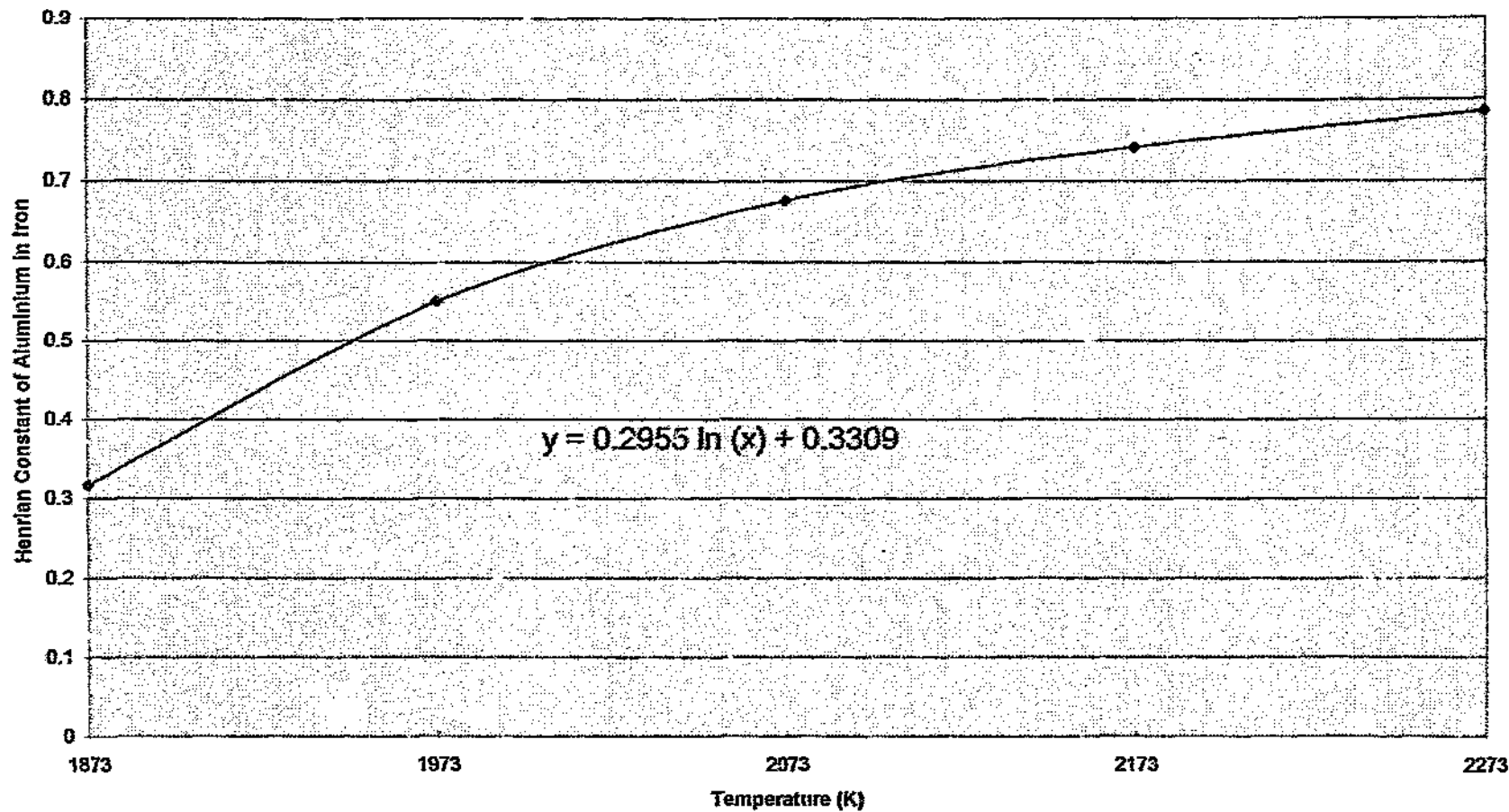
Figure 2.7 HENRIAN CONSTANT OF ALUMINIUM IN Fe-C-AI SYSTEM
