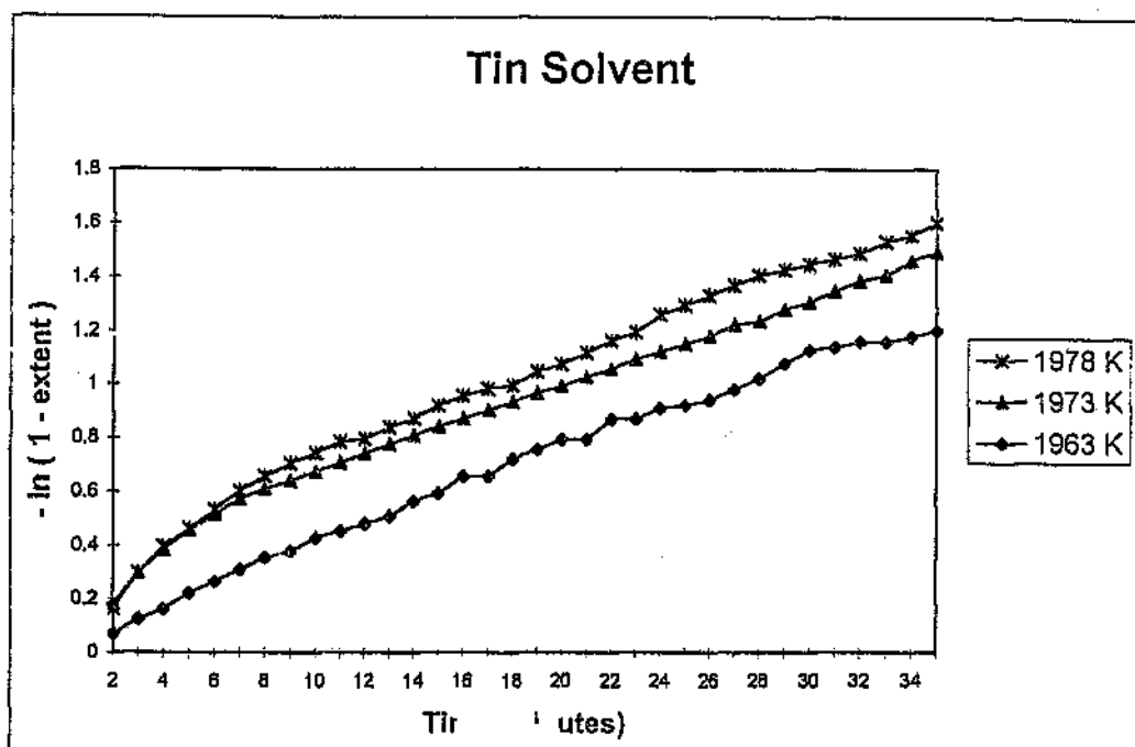
Figure 4.10 Extent of Reaction vs. Time in Tin Solvent
