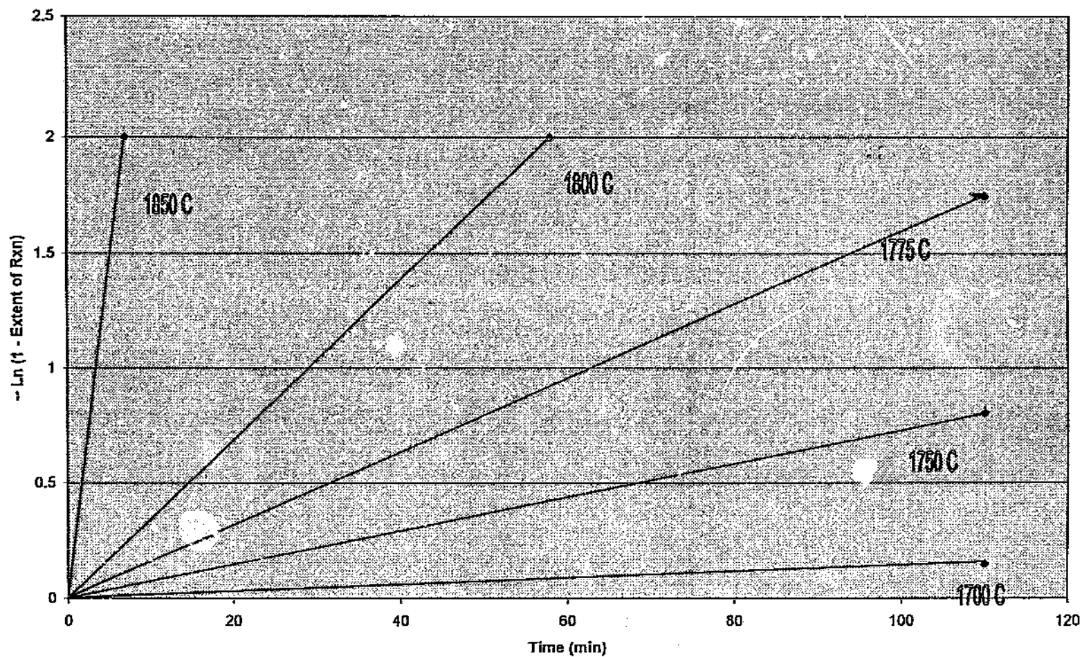
FIGURE 2.4 EFFECT OF TEMPERATURE ON REACTION RATE
