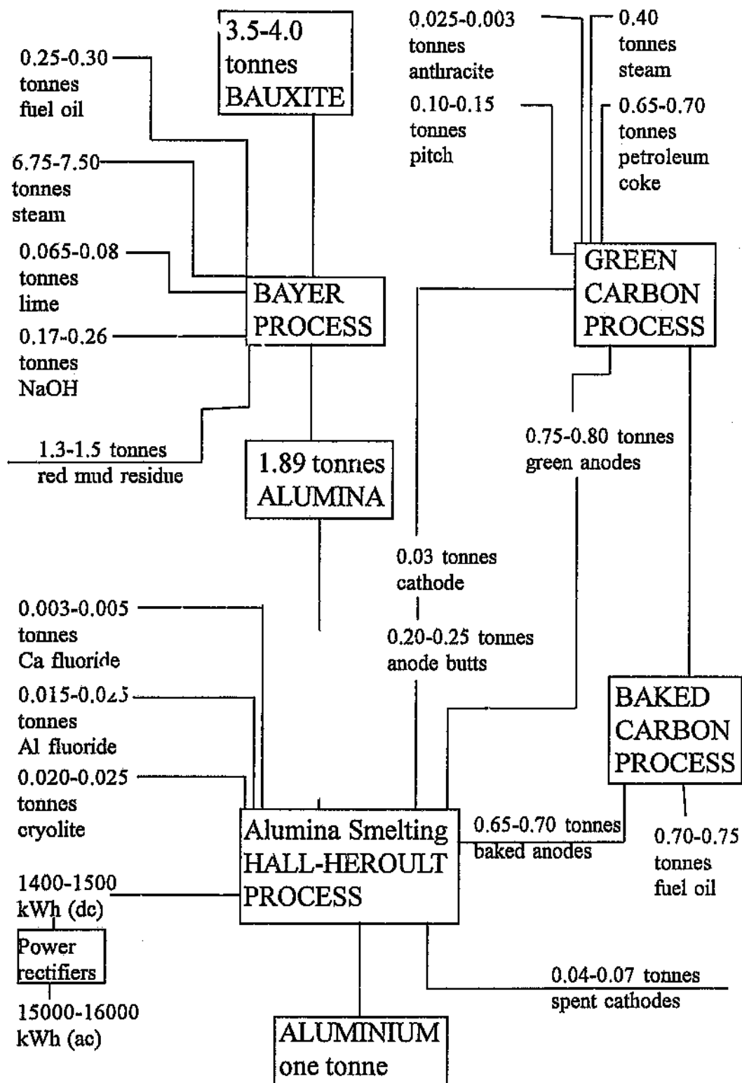
Figure 2.2 Integrated Al Flow Diagram (Australian Al Development Council)
