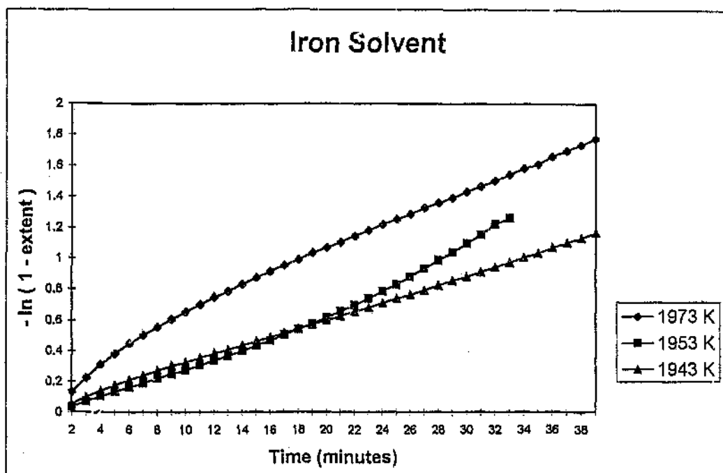
Figure 4.9 Extent of Reaction vs. Time in Iron Solvent
