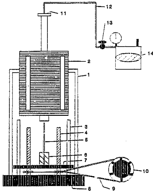
Figure 3.1 Furnace Set-up
