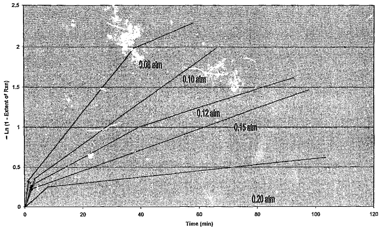
Figure 2.5 EFFECT OF PRESSURE ON REACTION RATE
