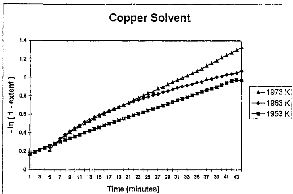
Figure 4.8 Extent of Reaction vs. Time in Copper Solvent
