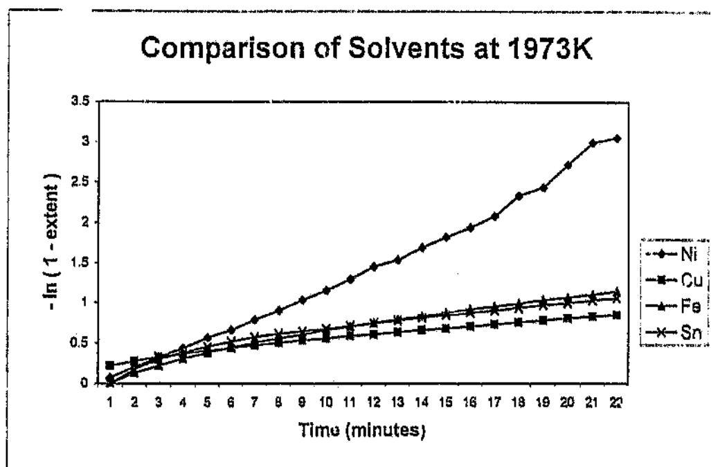
Figure 4.11 Extent of Reaction vs. Solvent Type at 1973K
