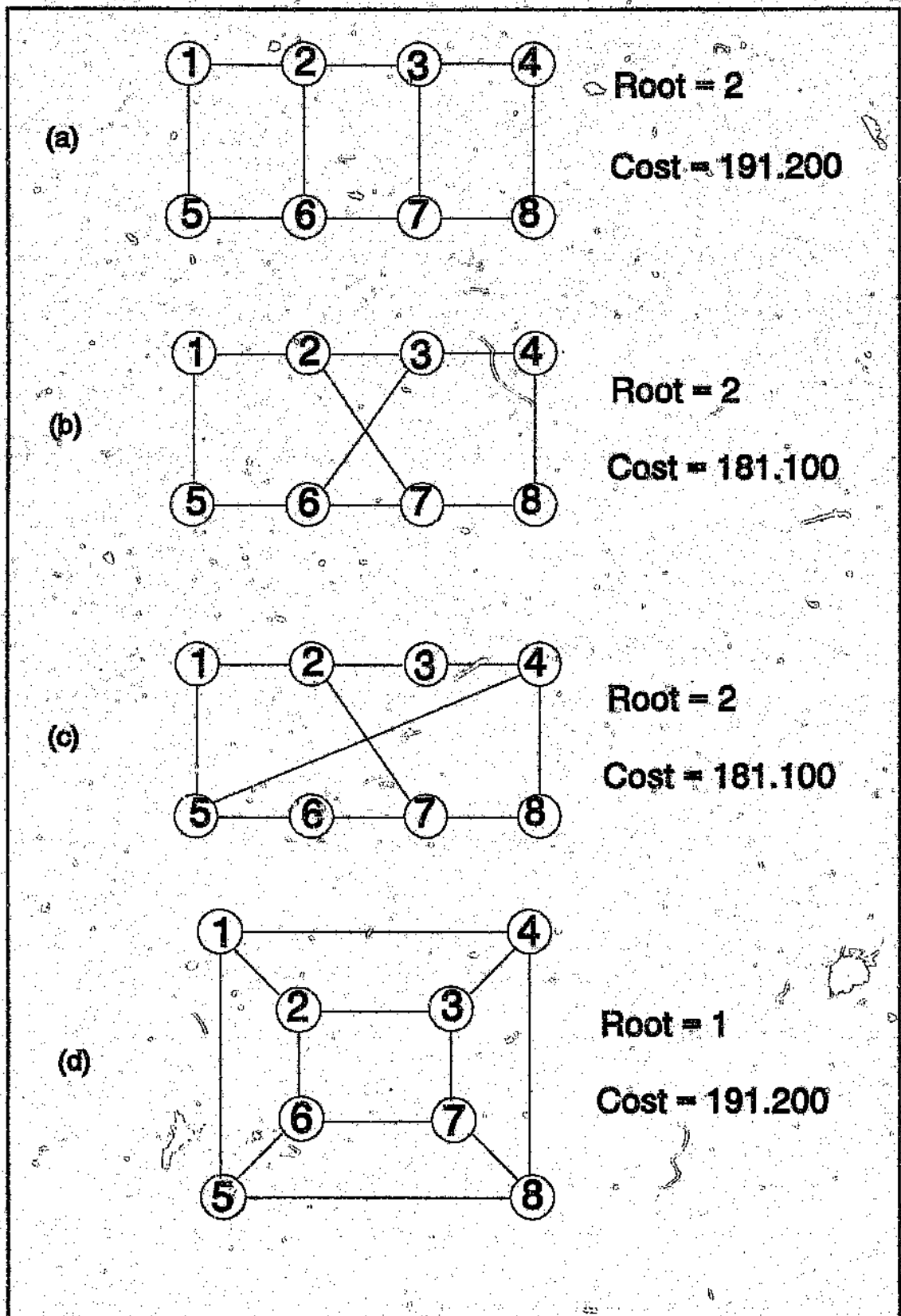
Figure 5.3 Various Topologies of an 8-bridge Internetwork
